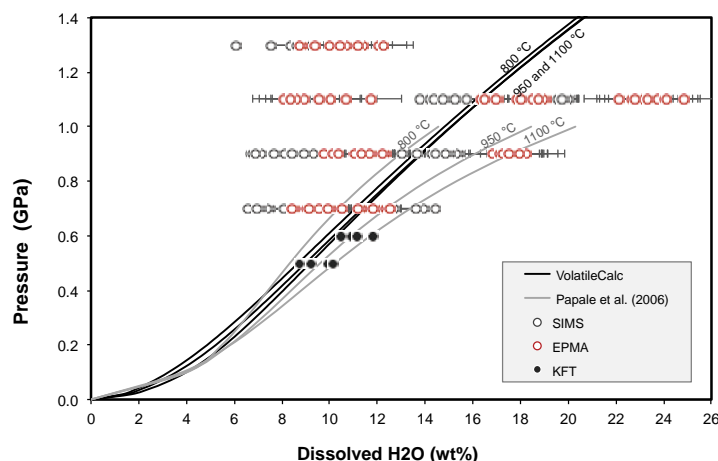
Figure 1. Pressure versus H 2 O content of glasses from solubility experiments, measured by SIMS, EPMA, and KFT. Water contents have been corrected for quench vesiculation using an appropriate equation of state, assuming a pure water vapour. Modelled H 2 O solubility curves from [3] and [4] are shown for reference.
