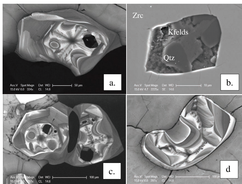
Fig. 1. CL (a, c, d) and SEI (b) images of zircon features in KUL. (a) shows the typical internal features of a zircon with a ‘complete’ core region and outer planar-zoned material, with some invasion of one sector by lobe of modified zircon, circular zircon in another sector, and a preserved former melt inclusion in another. (b) shows a nanogranite inclusion. (c) shows two grains welded together along a dissolution-reprecipitation front. (d) shows a composite of possibly 3 zircons (indicated by the trellis features) highly modified by invasive lobes.
