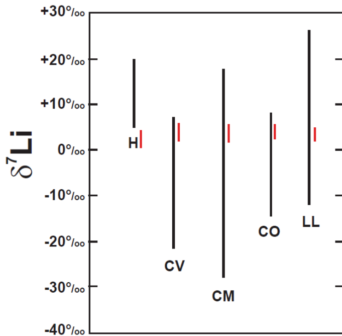
Figure 1. \delta^7\text{Li} ranges for analyses of chondrule phenocrysts from this study (black lines) versus corresponding bulk-rock measurements red lines [11]
