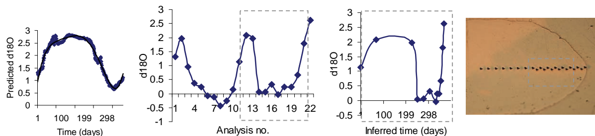
Fig. 4 \delta^{18}\text{O} profiles for a female plaice tagged by DST (pit marks shown in photograph). The predicted \delta^{18}\text{O} profile (left) is based on the DST-recorded temperature for this fish and an assumed constant salinity of 35 PSU. This predicted profile was used to modify the x-axis of the measured profile (centre) to give an inferred timeline for the experimental period (right). Note that unlike Figures 2 & 3, time is displayed from left to right.
