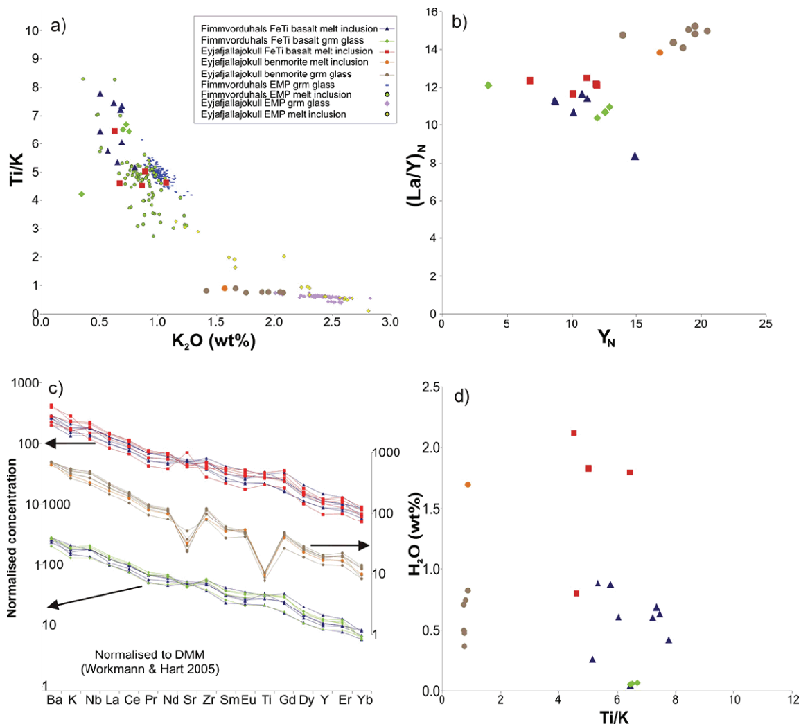
Fig. 1 Major, trace and volatile element concentrations, ratios and patterns in groundmass glass (grm) and plagioclase-hosted melt inclusions as measured by the ion probe in tephra samples from the 20 March to 12 April 2010 Fimmvörðuháls mildly alkalic (FeTi) basalt flank and 14 April to 22 May 2010 benmorite summit eruptions at Eyjafjallajökull volcano (Iceland). See key for further details. (a) TiO 2 /K 2 O versus K 2 O (wt%). The compositional fields of groundmass glass and melt inclusions as determined by electron microprobe (EMP) in samples from both eruptions is shown for comparison. (b) Rare earth element fractionation as illustrated by (La/Y) N versus Y N (ppm). (c) Normalized multi-element diagram showing fractionation patterns for (i) basalt groundmass glass and melt inclusions from Fimmvörðuháls flank eruption (lowest panel), (ii) benmorite groundmass glass and melt inclusion from the summit eruption (middle panel), and (iii) plagioclase-hosted basalt melt inclusions from the summit and Fimmvörðuháls events (top panel). Trace element concentrations are normalized to depleted mantle (DMM) values [3]. (d) Water concentrations versus Ti/K in melt inclusions and groundmass glass from both eruptions.
