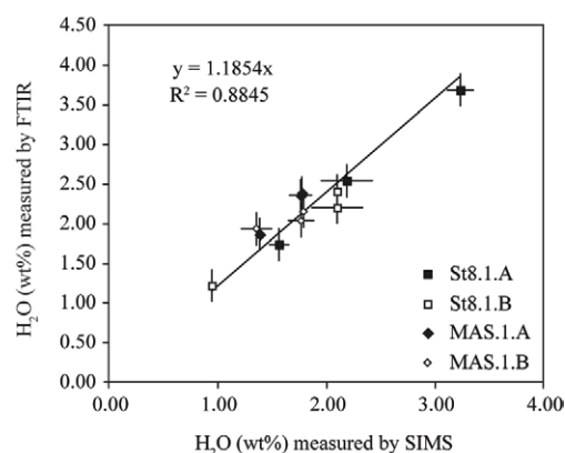
Figure 4. Comparison of H 2 O contents of experimental glasses measured by both FTIR and SIMS. Deviation from a 1:1 line is attributed to uncertainty in the extinction coefficient used for processing FTIR data. A correction factor of 1.1854 has been applied to all of the FTIR data to bring them into line with SIMS. No such correction was required for CO 2 data.
