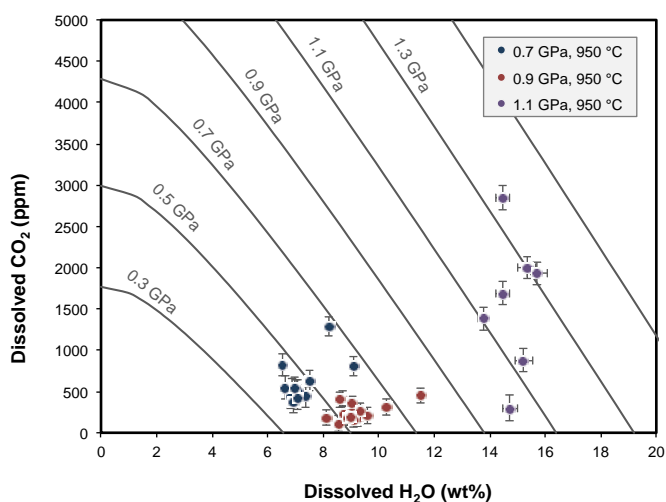
Figure 2. H 2 O and CO 2 contents of three experimental glasses measured by SIMS, plotted against modelled solubility isobars [3]. These runs were intended to be CO 2 -free, but carbon is clearly present. CO 2 contents inferred from carbon measurements are variable within each sample and range from hundreds to thousands of ppm.
