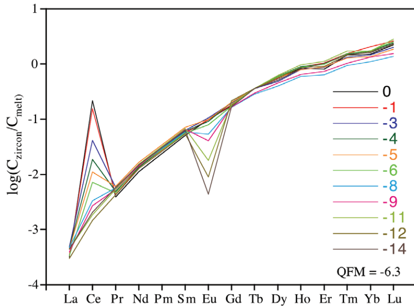
Figure 2: Average REE zircon-melt partition coefficients as a function of oxygen fugacity. The REE patterns have been referenced to Tb to aid comparison.
