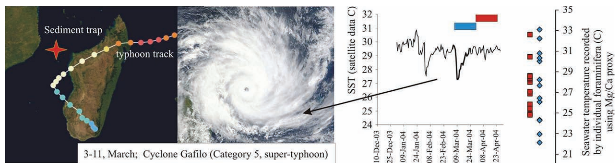
Fig. 2 Left: Location of the sediment trap, track and satellite image of the Cyclone Gafilo passed in Madagascar area during March 2004. Note that scale on both images is approximately the same. Right: Variation in sea surface temperature at sediment trap site recorded by satellite. Bold line marks time of the cyclone activity in this area. Blue and red rectangles correspond to two sediment trap collection intervals of foraminiferal samples analysed using SIMS. The small red squares and blue diamonds (13 shells each) represent temperatures recorded by individual foraminifera based on their Mg/Ca ratios. Note that most of the red symbols are tightly group around 25-29°C temperature range whereas blue symbols (foraminifera collected during cyclone activity) are spread along a 22-33°C interval reflecting a significant increase in variability.
