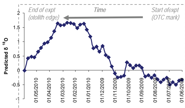
Fig. 2 Predicted \delta^{18}\text{O} data for experimental plaice maintained at the CEFAS aquarium for 12 months from June 2009. The prediction is based on an equation derived from experimental work with juvenile North Sea cod ( I. ). In all figures in this report, the dotted line box indicates the period of interest (aquarium or DST experiment) and the shaded boxes indicate inferred seasons (summer: orange, winter: blue).
