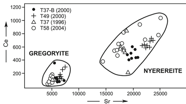
Fig. 4. Ce and Sr compositions of gregoryite and nyerereite
