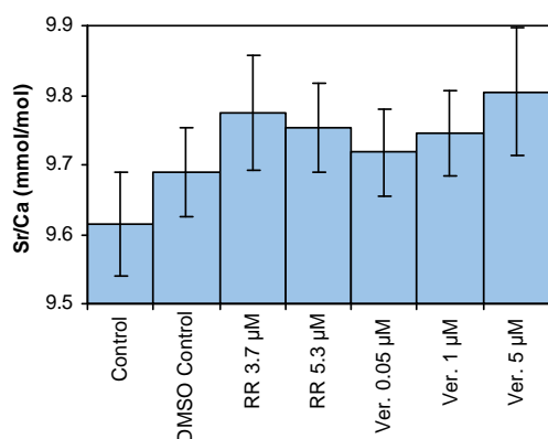
Figure 1. Mean Sr/Ca of coral aragonite deposited in each treatment. Error bars indicate 95% confidence limits ( 2\sigma/\sqrt{n} ). RR = ruthenium red. Ver. = verapamil.
