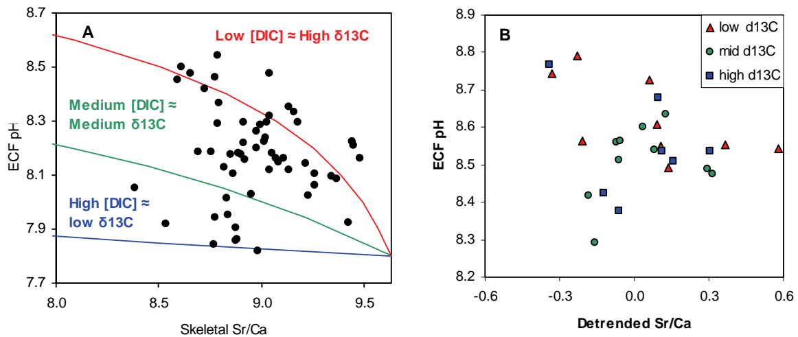
Figure 2. A: Modeled skeletal Sr/Ca as a function of ECF pH under a range of DIC scenarios. Green line shows [\text{CO}_2] in the overlying coral tissue is ambient i.e. maintains equilibrium with atmospheric \text{CO}_2 levels. At low DIC tissue [\text{CO}_2] is ambient/5 and at high DIC tissue [\text{CO}_2] is ambient x5. Black dots represent observed SIMS data. B: Observed detrended skeletal Sr/Ca and ECF pH (estimated from skeletal \delta^{11}\text{B} ), divided into groups of low, mid and high \delta^{13}\text{C} values. \delta^{13}\text{C} is detrended to remove the seasonal signal which may reflect seasonal variations in \delta^{13}\text{C} of seawater or in the \delta^{13}\text{C} of metabolic \text{CO}_2 (4).
