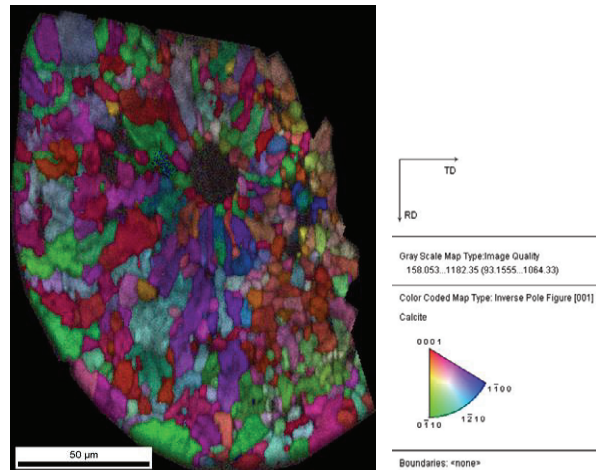
Fig. 2: Diagenetic alteration of O. umbonatus analysed by EBSD (site 1221C 11X3 2-3cm) which shows pattern indicative of recrystallisation.
