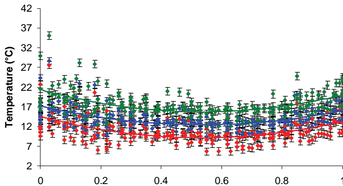
Figure 2: Temperature profiles of all fish combined using a derived equation (red), Storm-Suke et al. (blue) and Kim et al. (green) scaled by proportionate distance in the marine zone of the otolith
