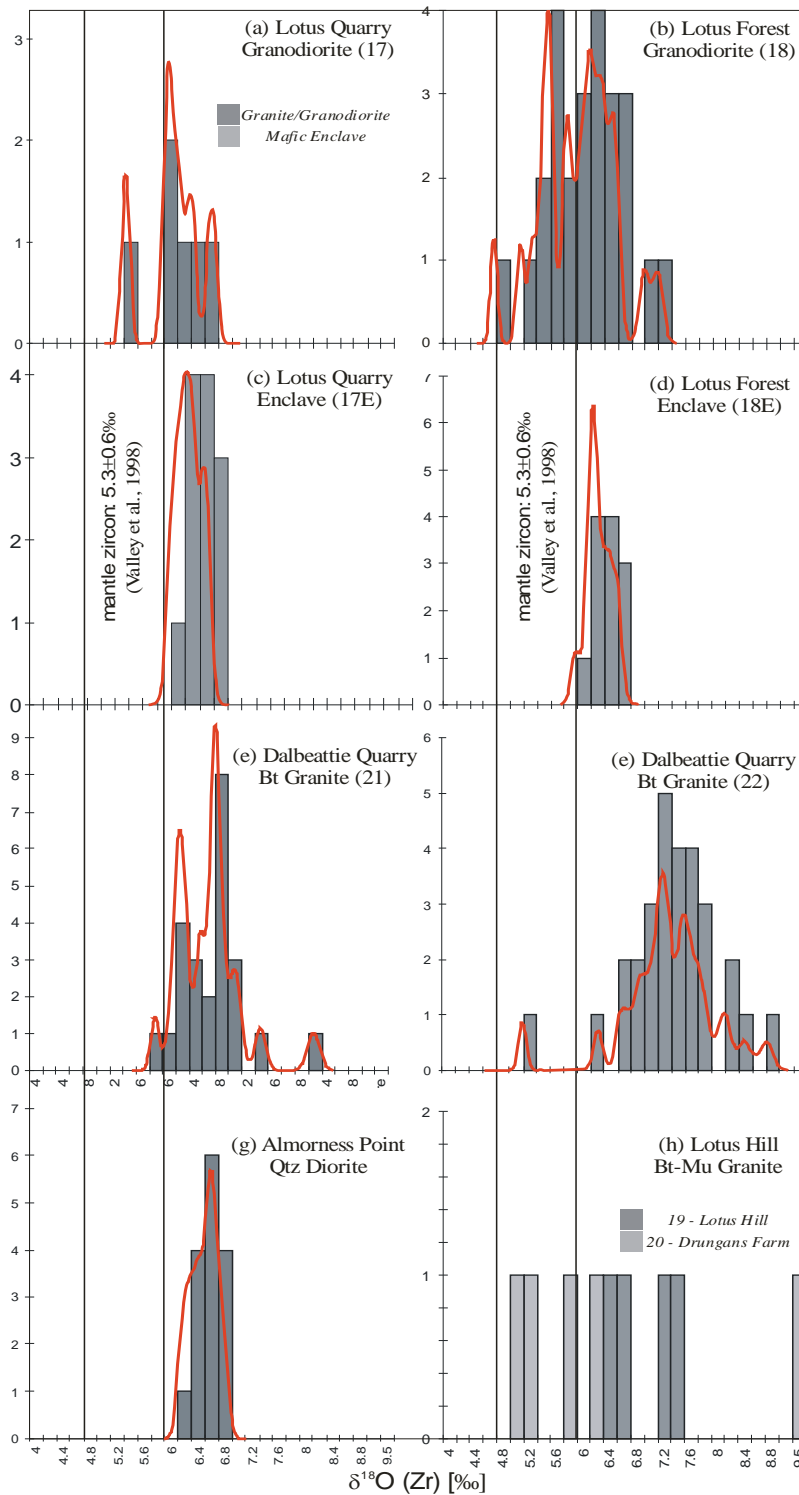
Fig. 1 Zircon oxygen isotope compositions for the outer- to inner-most zones 1 (sample 17), 2 (sample 18), 3 (sample 21), 4 (sample 22) and 5 (samples 19 and 20). Mean oxygen isotope compositions increase systematically from outer to inner zones, with an increase in the width of the associated probability distribution. Also shown are the oxygen isotope compositions of zircons from two mafic enclaves from zones 1 and 2 (17E and 18E respectively) and the marginal quartz diorite.
