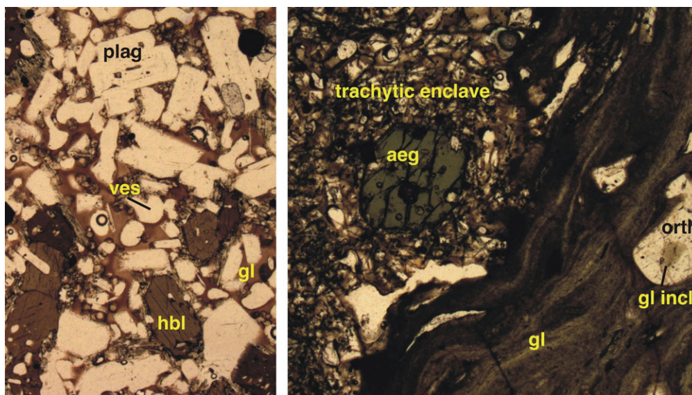
Figure 1. Left: Basaltic andesite enclave in Soufriere Hills Volcano andesite (glass is rhyolitic). Right: Trachytic enclave in peralkaline rhyolite from Pantelleria. Labels plag (plagioclase), ves (vesicle), gl (glass), hbl (hornblende) aeg (aegirine-augite), orth (orthoclase), gl incl (glass inclusion).
