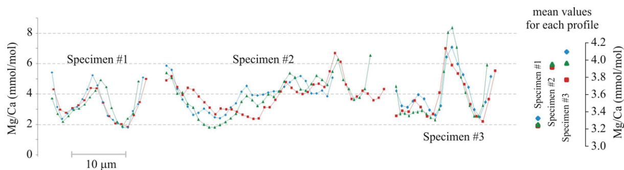
Fig. 1 Reproducibility of Mg/Ca measurements of G. sacculifer final chambers using SIMS 1- \mu\text{m} step profiling across the chamber cross-section. Three replicate profiles (marked by coloured symbols) show reproducible Mg/Ca patterns and average Mg/Ca values for each specimen (indicated on the right).
