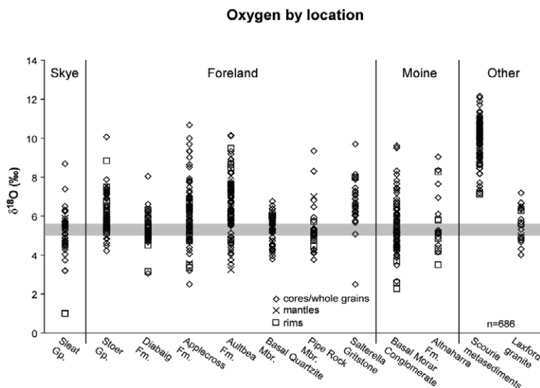
Figure 1. All oxygen analyses sorted by sample (in stratigraphic order) and zircon growth zone. Diamonds - cores and whole grains; crosses - mantles; squares - rims. Grey bar indicates expected range of oxygen values in zircons crystallising directly from mantle material.
