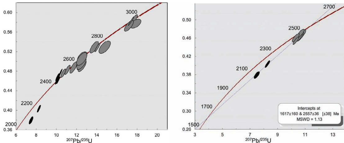
Fig. 1 A) (left) Concordia plot (Isoplot v3.0) showing data points from undeformed (grey) and deformed (black) zircons; B) (right) Concordia plot of zircon data from one sample with a Discordia line plotted through deformed zircon data points; the lower intercept age is interpreted to be the age of the zircon lattice deformation
