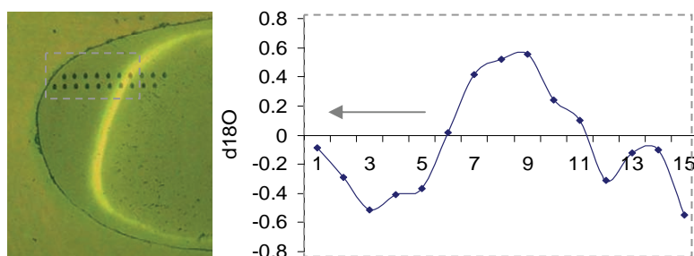
Fig. 3 \delta^{18}\text{O} profile for a female plaice maintained at CEFAS for 12 months. The photograph shows the otolith pit marks and the OTC (yellow) mark indicates the experiment start point. The graph shows \delta^{18}\text{O} values for the experimental period. The arrow indicates particularly fast growth post-spawning.
