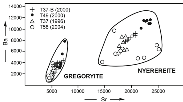
Fig. 3. Ba and Sr compositions of gregoryite and nyerereite
