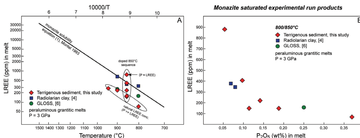
Figure 1A. Undoped experiments have lower apparent monazite solubilities than predicted using Montel [2]. We also find strong very variable monazite solubilities depending on how much \Sigma LREE was initially added to our starting materials (850°C sequence and other shown experiments). 1B) Inverse LREE/P correlation suggests that monazite solubility is dependent on P in the melt.
