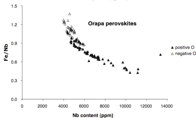
Fig 2: Variation of Nb concentration between two groups of Orapa perovskites with different \delta^{18}\text{O} values.
