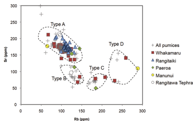
Fig. 2: Trace element variation in Whakamaru pumices (whole-rock XRF data), showing chemical variation within and between ignimbrite units– indicating four discrete magma batches (type A-D).
