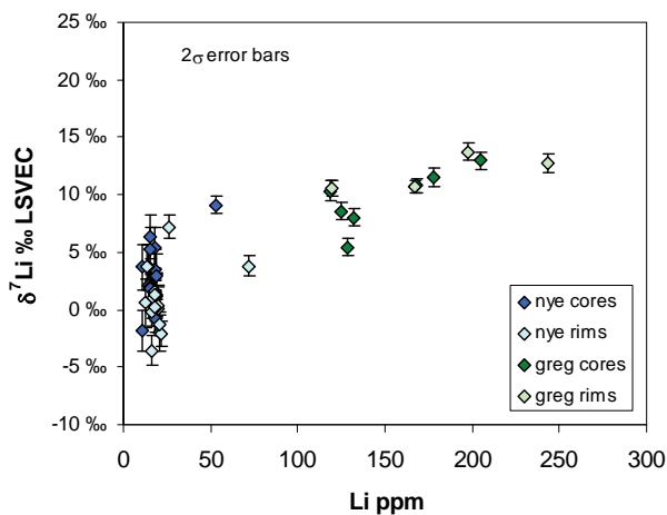
Fig. 5. Li isotope systematics of gregoryite and nyerereite cores and rims.
