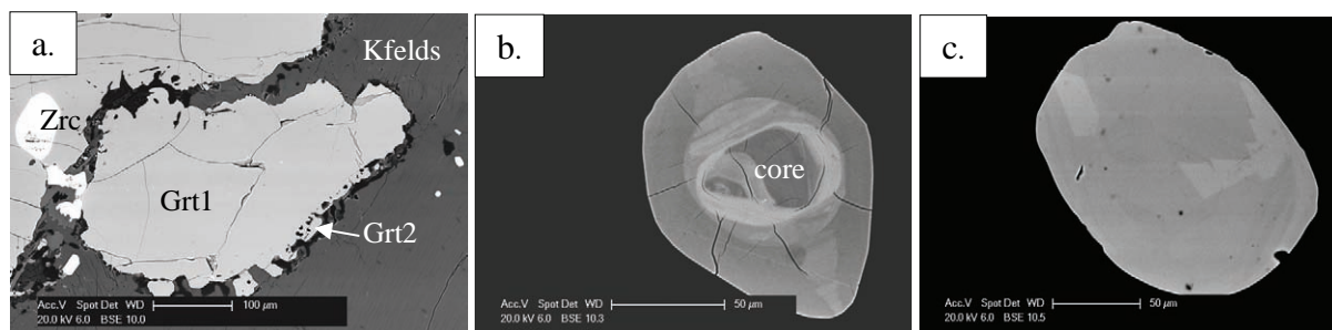
Fig. 1. BSE images of garnet (a) and zircons (b, c) in the EGB leucogranite. Notice the small relict zircon cores seen in b) and the weakly-developed fir tree zoning in c). The zircon shown in c) has a ^{206}\text{Pb}/^{207}\text{Pb} age of c. 922 Ma.
