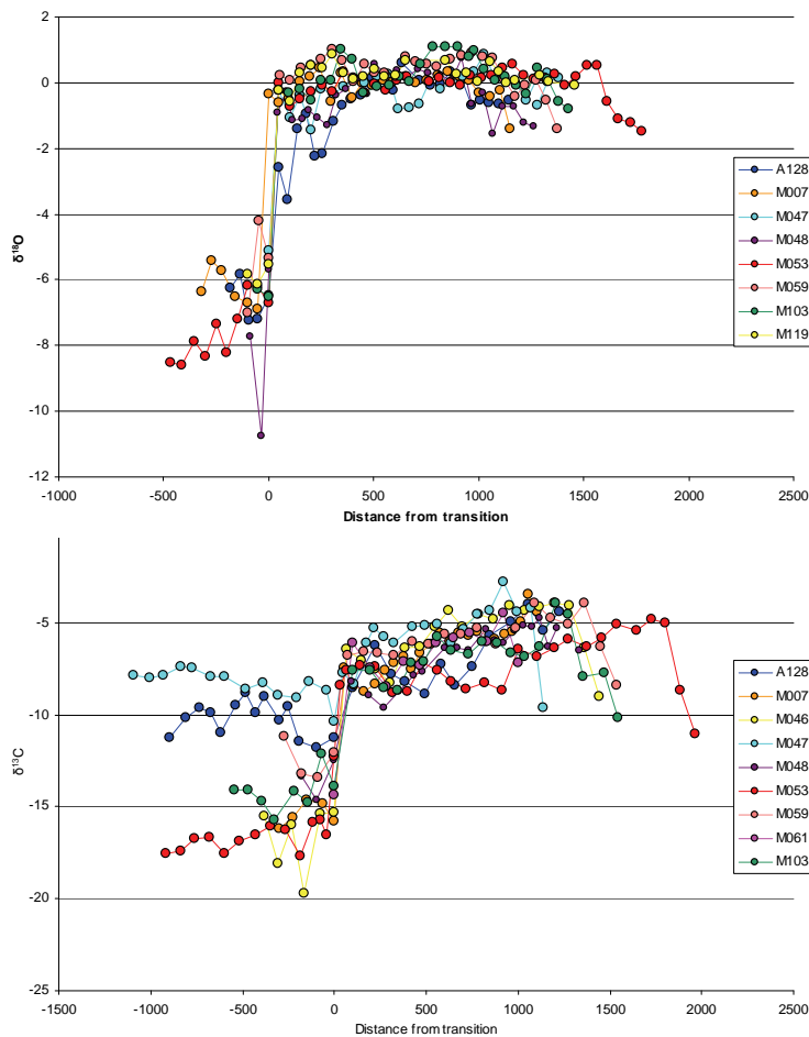
Figure 1: \delta^{18}\text{O} ( top ) and \delta^{13}\text{C} ( bottom ) profiles from the fresh-water/marine transition and marine zone of 1SW wild Atlantic salmon otoliths ( n = 8 individuals for oxygen and n = 9 for carbon). Analytical precisions were better than 0.21‰ and 0.43‰ respectively.
