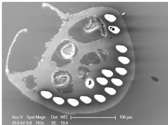
Fig. 1: SEM image of O. umbonatus from Central Exmouth Plateau (762) analysed by Cameca 1270 for \delta^{11}\text{B} .
