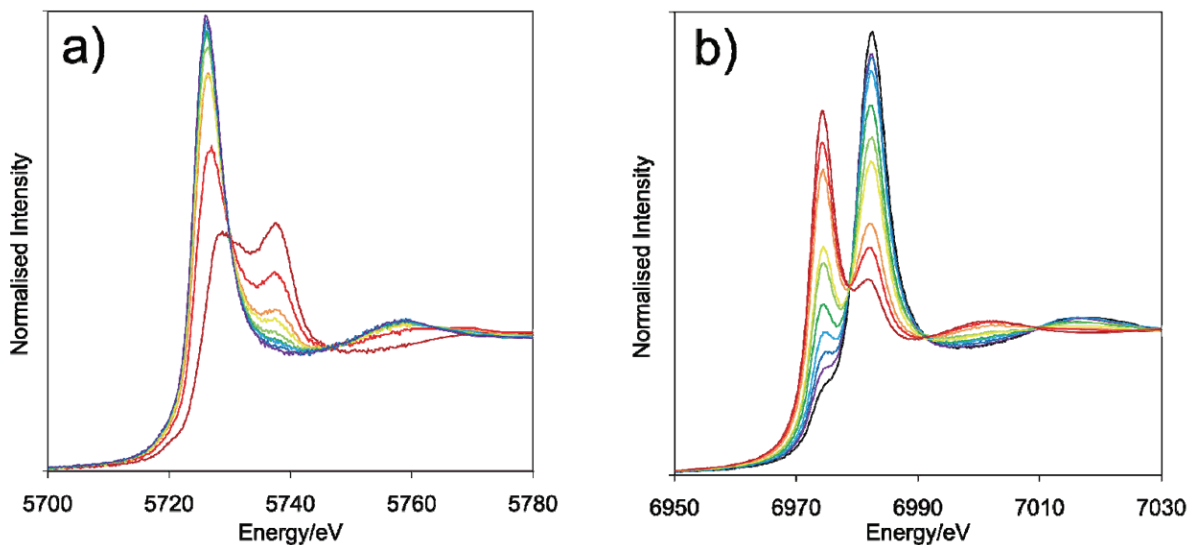
Figure 3: a) Ce and b) Eu XANES spectra of silicate glasses that were equilibrated as melts over a range of f\text{O}_2 s.
