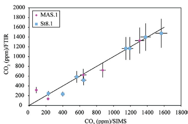
Figure 3. Comparison of CO 2 contents of experimental glasses measured by both FTIR and SIMS. Deviation from a 1:1 line is attributed to uncertainty in the extinction coefficient used for processing FTIR data.
